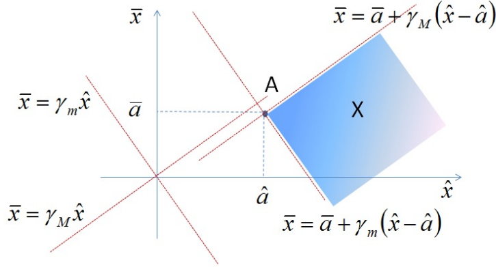
Figure 2: the set of intervals \mathbb{D}_{\gamma_m, \gamma_M}(A)
