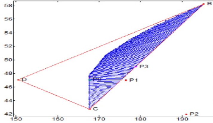
Figure 9: Numerical example from Sengupta and Pal
