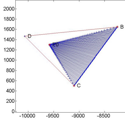
Figure 5: the ideal and the optimal solution of example 1 are shown
