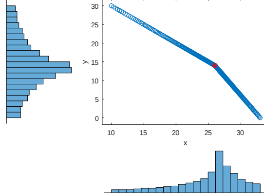
Figure 6: sensitivity analysis for example 1
