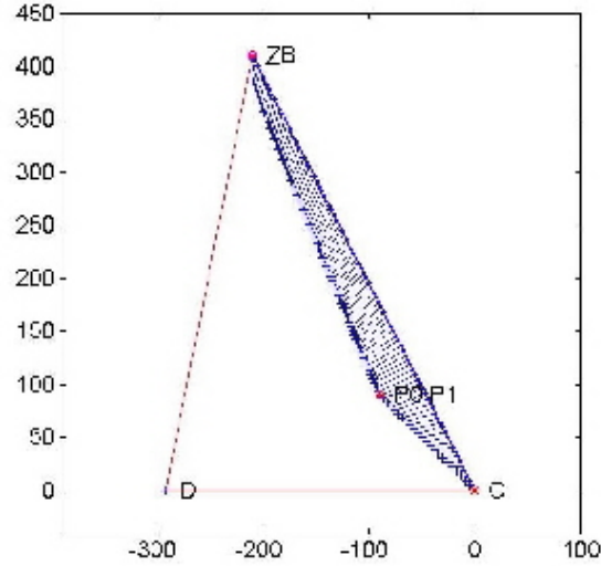
Figure 7: Numerical example from Chanas and Kuchta with \gamma_m = 0 , \gamma_M = 5.0
