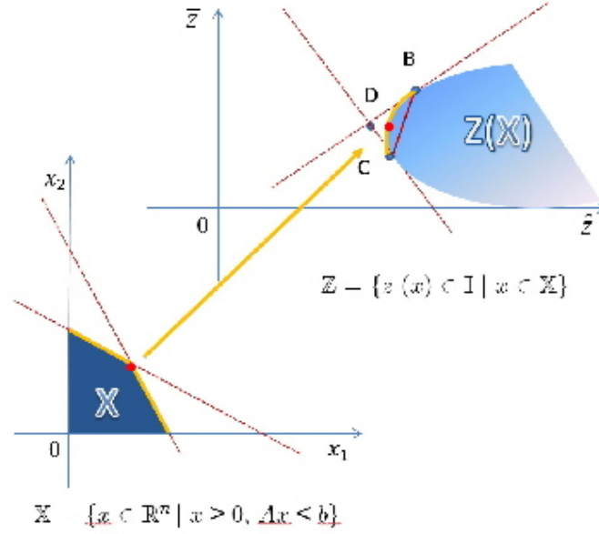
Figure 3: from the feasible convex set to the feasible objective intervals
