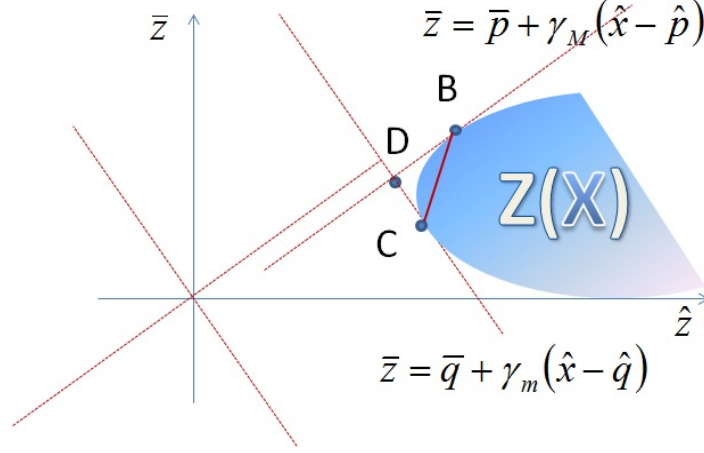
Figure 4: tangent lines to \mathbb{Z}
