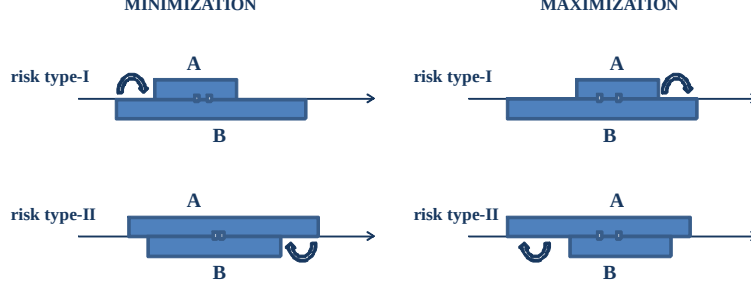
Figure 1: type-I and type-II risks that may occur in minimization and maximization problems.
