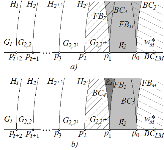
Figure 7: A neighborhood of the curve BC_{LM} shown schematically near the border-flip point p_0 . The flip bifurcation at FB_M is subcritical in a ) and supercritical in b ). The point p_1 is also a border-flip codimension-two bifurcation point.
