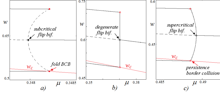
Figure 3: 1D bifurcation diagrams illustrating subcritical a) , degenerate b) and supercritical c) flip bifurcation of the fixed point w_M^* . Here m = 1.2 and \alpha = 0.47 , \beta = 2.25 in a) , \alpha = 0.5 , \beta = 2.25 in b) , \alpha = 0.6 , \beta = 2 in c) .
